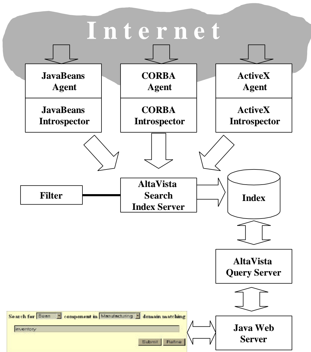
Figure 2: Agora Architecture
