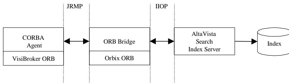
Figure 6: ORB Bridge
